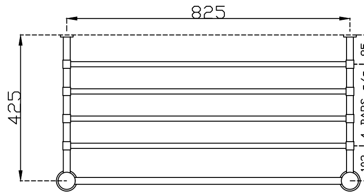
METAL FRAME VIEW
